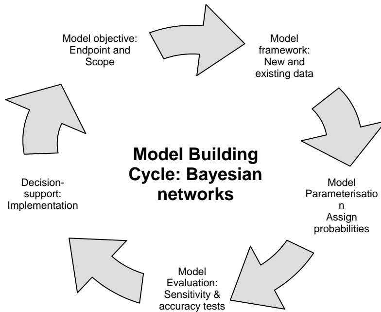
Figure 2: Steps followed in building a Bayesian network.
